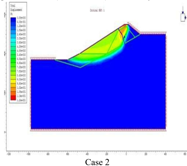
Figure 4: Evaluation of Phase 2 stress in Case 2 (Rapid Drawdown)
