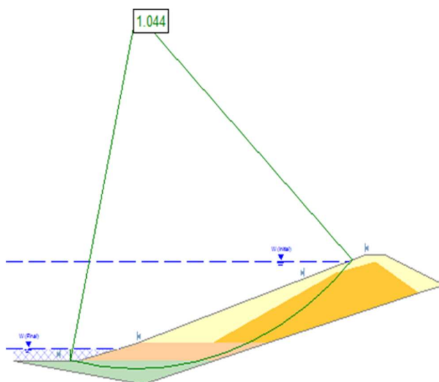
Figure 5: Drawdown case stability analysis for Rocscience Slide-6.0
