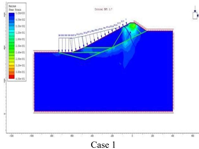
Figure 3: Case 1 (full reservoir) stress analysis in Phase 2
