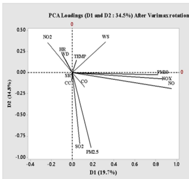
Figure 8 shows the PCA loading for Cluster 2.
