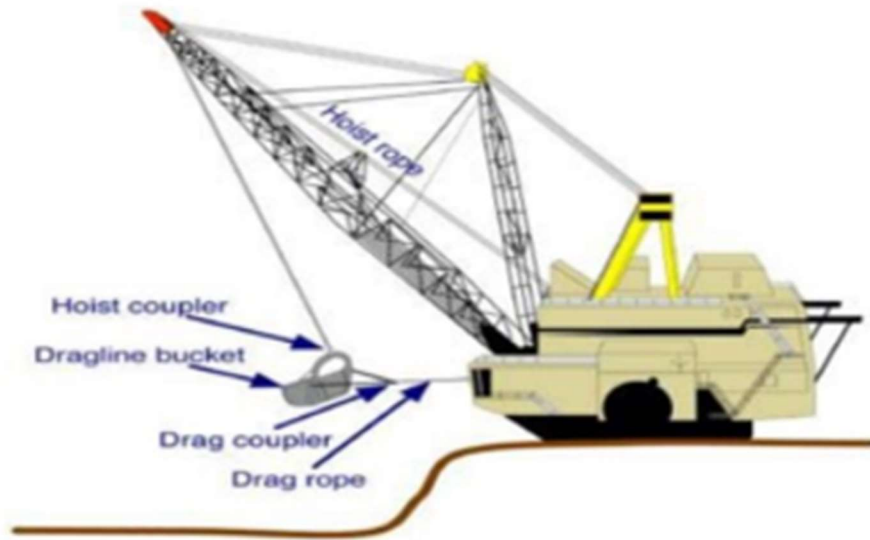
Fig-1:walking dragline
